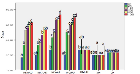
Figure 8: Lethality after 24 h exposure
