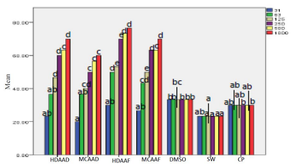
Figure 9: Lethality after 36 h exposure
