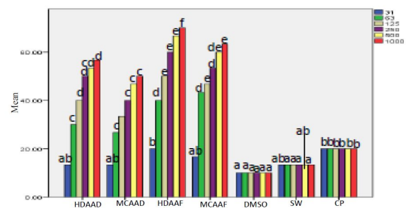
Figure 7: Lethality after 12 h exposure
