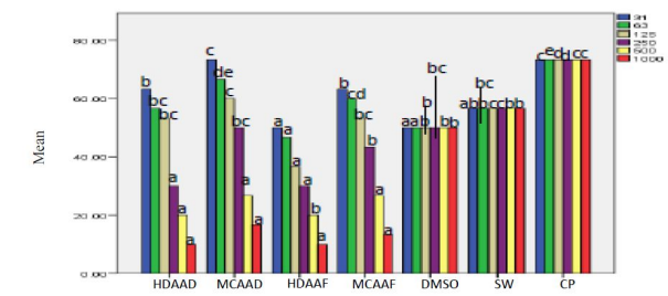
Figure 3: Hatchability after 36 h exposure
