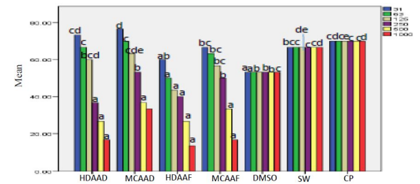
Figure 4: Hatchability after 48 h exposure
