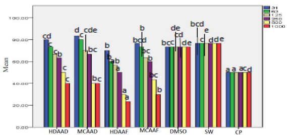
Figure 6: Hatchability after 72 h exposure
